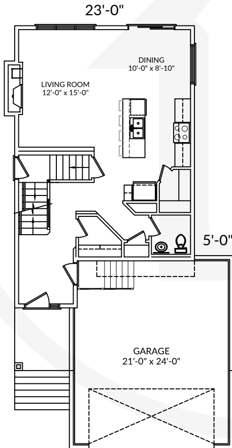
MAIN FLOOR PLAN (747 Sq. Ft.)
