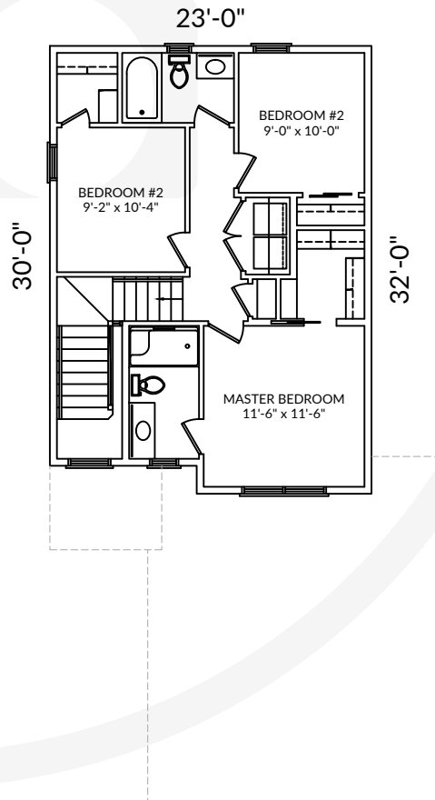
UPPER FLOOR PLAN (685 Sq. Ft.)
